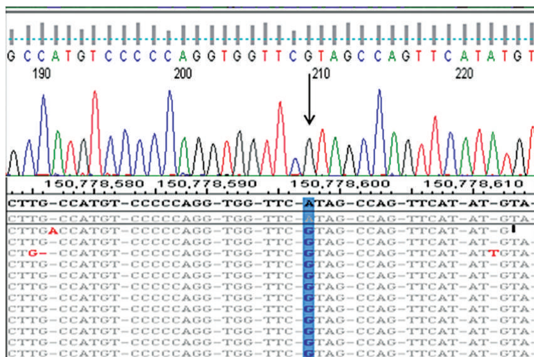
Figure 4. CTSK c.224T>C (p.Met75Thr) Sanger phrenogram and next-generation sequencing.
